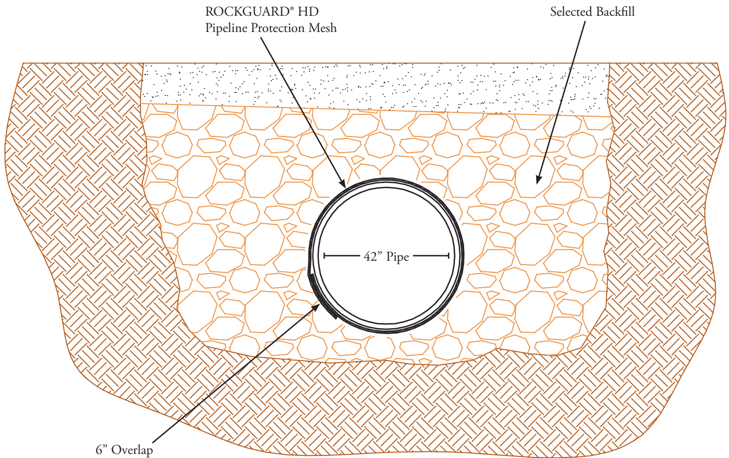
SECTION VIEW
